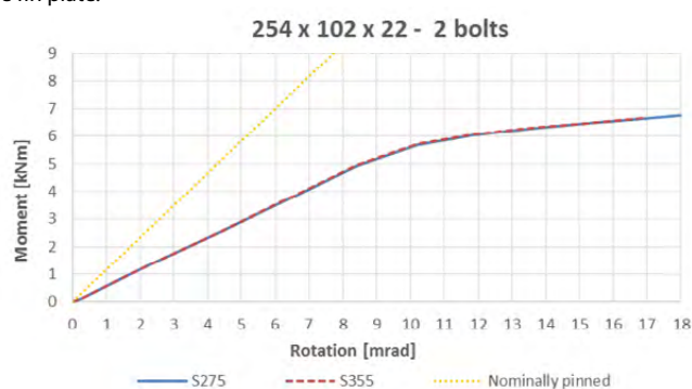
Figure 3: Moment-rotation curves for 254 \times 102 UB, 2 bolts
