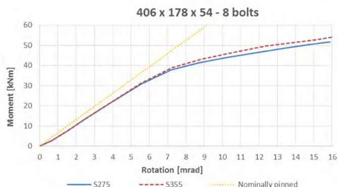
Figure 4: Moment-rotation curves for 406 \times 178 UB, 8 bolts
