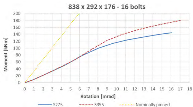
Figure 5: Moment-rotation curves for 838 \times 292 UB, 16 bolts
